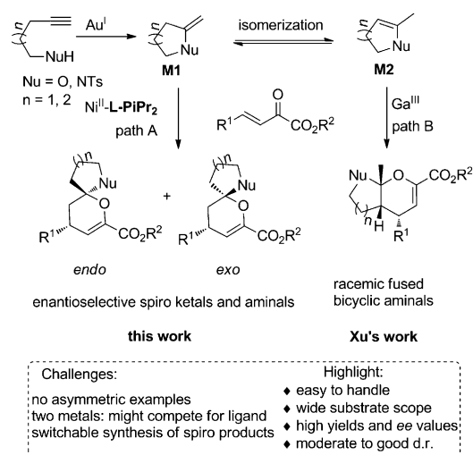
Scheme 1. Lewis acids catalysis combined with \pi -acid gold(I) catalysis (path A) compared to previous work by Xu and co-workers (path B; Ref. [13]). See Table 1 for the structure of L-PIPr 2 .
